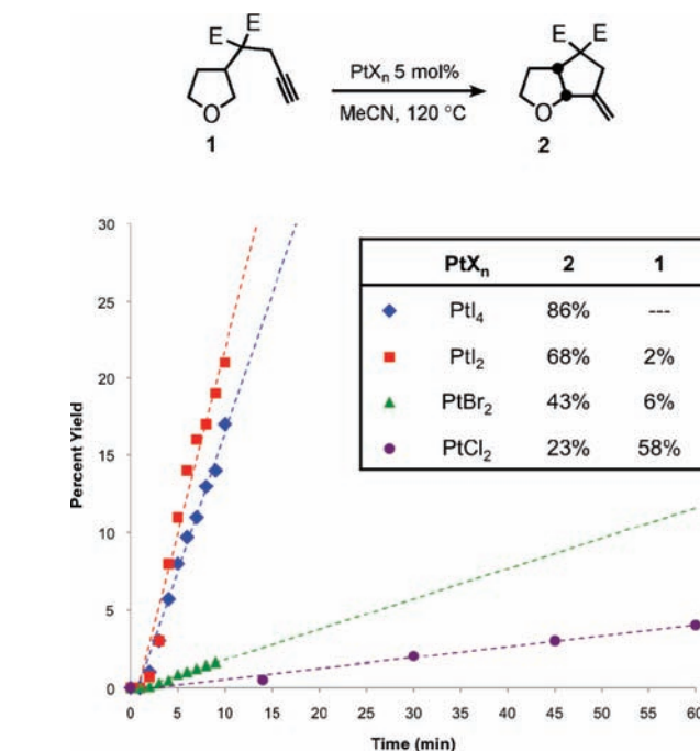
Figure 1. Effect of halide ligand on the catalyst activity. Initial rates of product 2 formation are shown in the plot. The inset lists the yields of product 2 and remaining starting material 1 . Reactions performed at 0.05 M in dry MeCN. Yields were determined by GC, employing tetrachlorobenzene as an internal standard. E = CO 2 Me.
